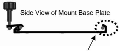
Position Large Flange Hook Forward on Boat
